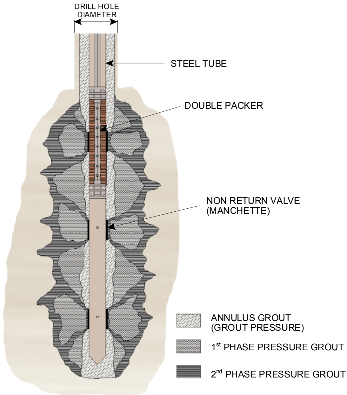
Figure 4-14. Use of Reinforcement Tube as a Tube á Manchette Postgrouting System.
